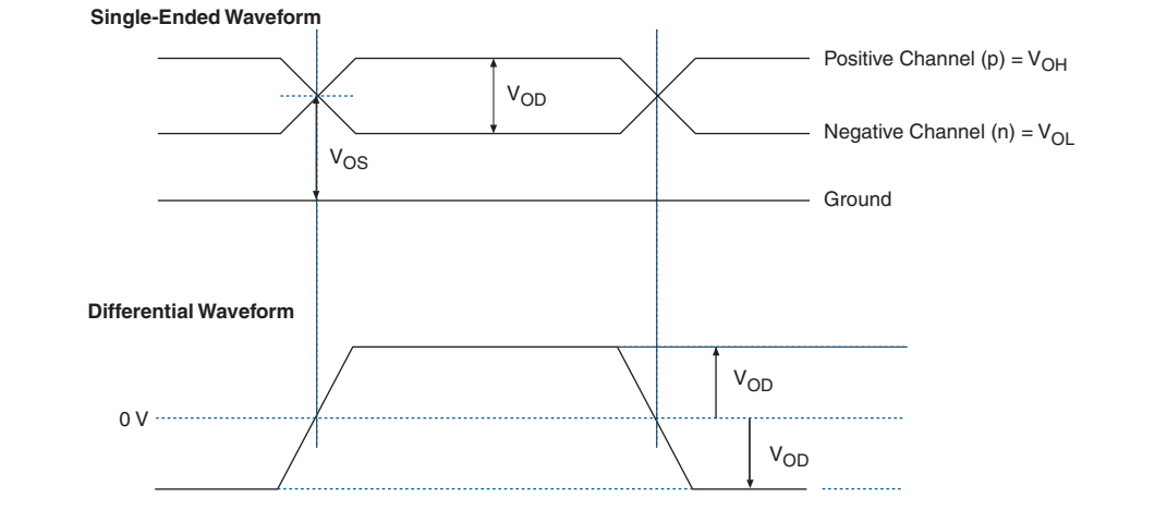
Figure 11-8. Transmitter Output Signal Level Waveforms for mini-LVDS
