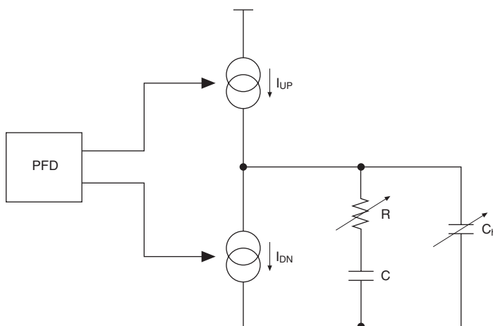
Figure 7-13. Loop Filter Programmable Components
