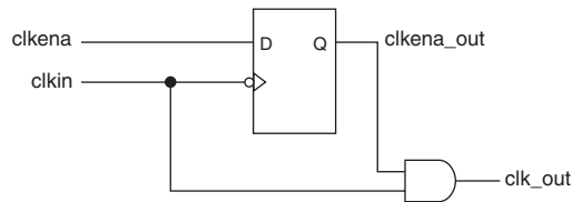
Figure 7-17. clkena Implementation
