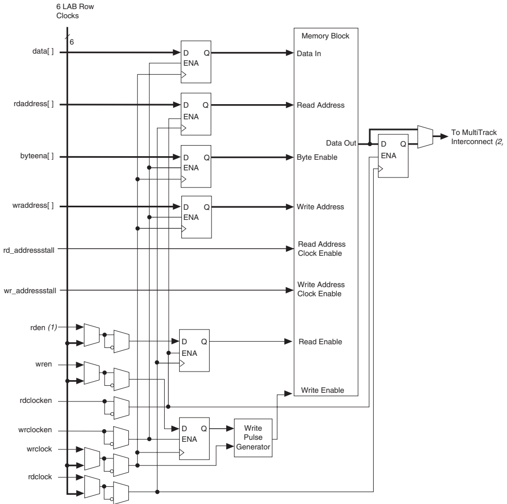
Figure 8–17. Cyclone II Read/Write Clock Mode
