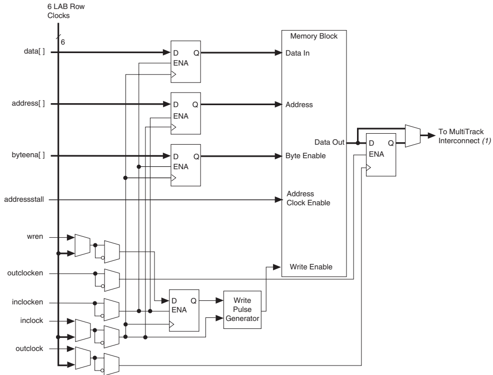
Figure 8–16. Cyclone II Input/Output Clock Mode in Single-Port Mode
