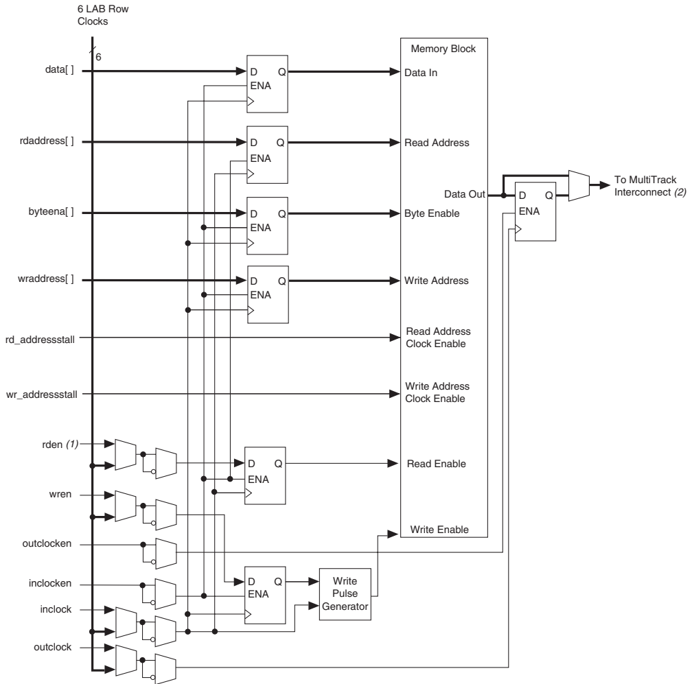
Figure 8–15. Cyclone II Input/Output Clock Mode in Simple Dual-Port Mode
