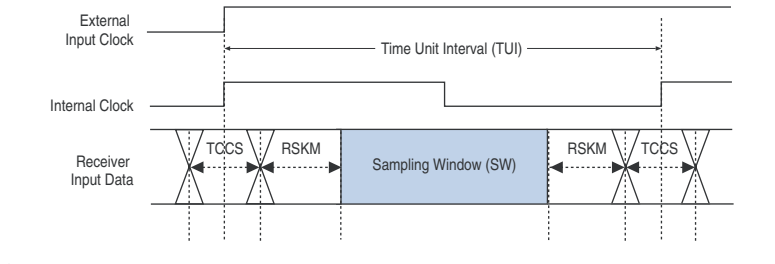
Figure 11-15. High-Speed I/O Timing Diagram
