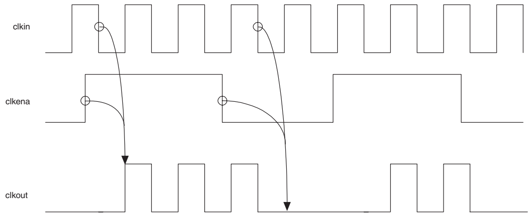
Figure 7-18. clkena Implementation
