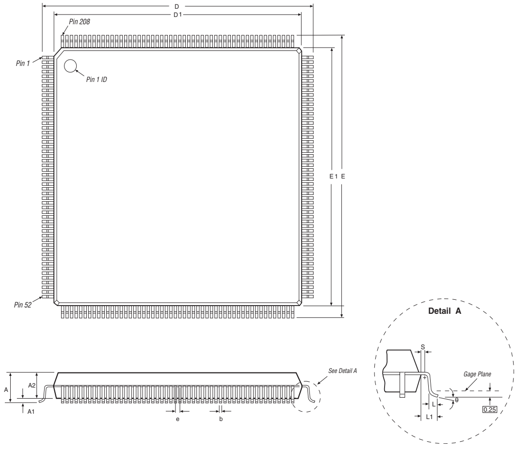
Figure 15–2. Package Outline for 208-Pin PQFP
