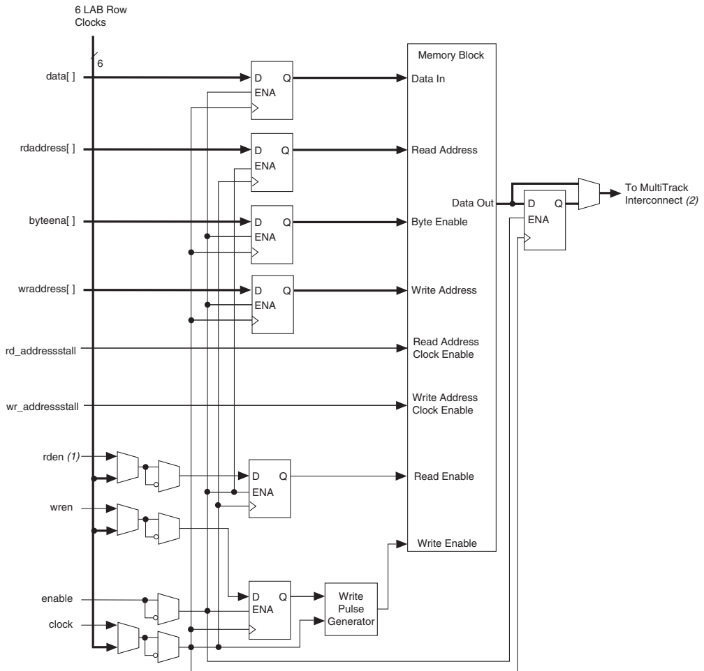
Figure 8–19. Cyclone II Single-Clock Mode in Simple Dual-Port Mode
