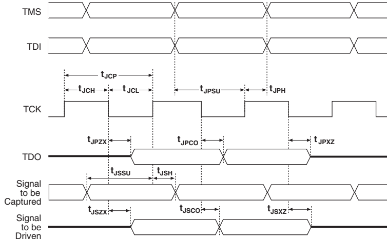
Figure 3–1. Cyclone II JTAG Waveform
