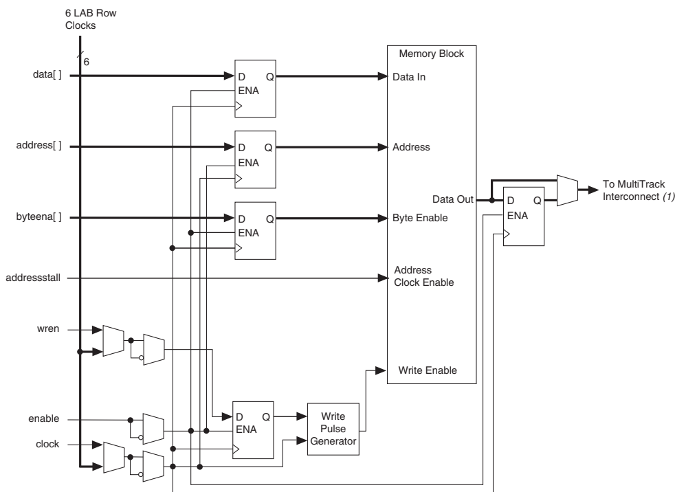
Figure 8–20. Cyclone II Single-Clock Mode in Single-Port Mode
