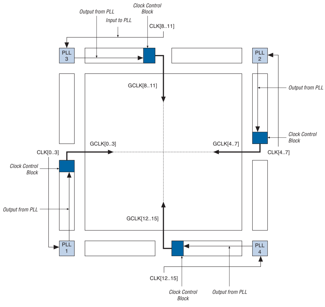
Figure 7–15. Cyclone II Clock Control Blocks Placement
